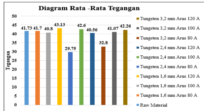
Gambar 24 Diagram Rata – Rata Tegangan
