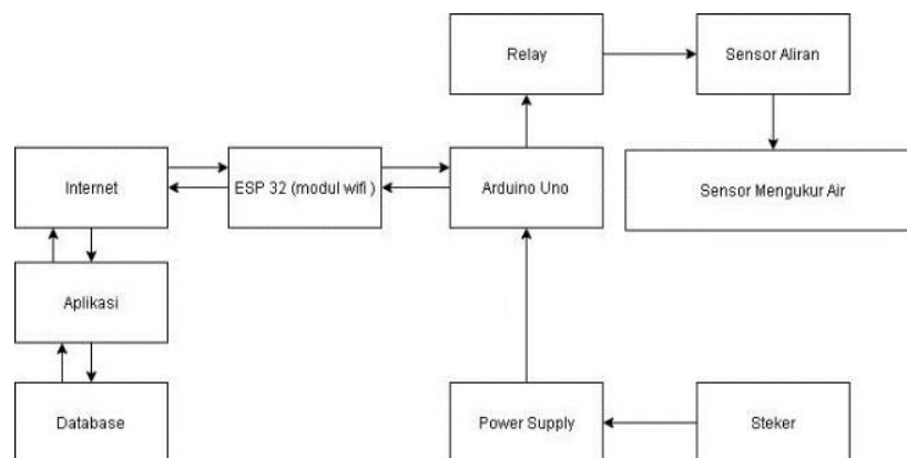
Gambar 2 Diagram Blok
