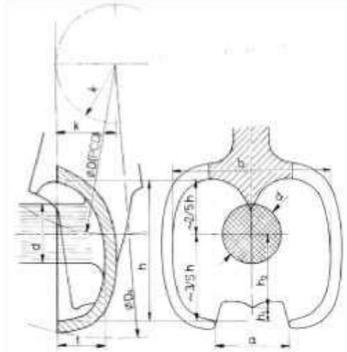
Gambar 1. Dimensi sudu turbin pelton (Eisenring, 1991)
