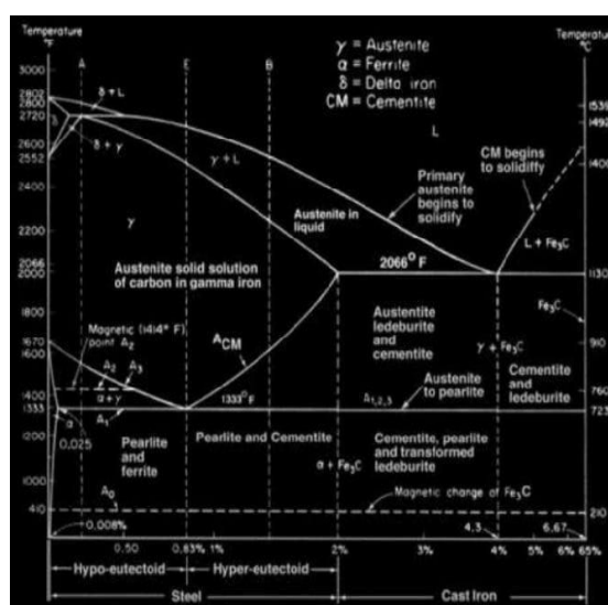
Diagram Fasa Fe-Fe 3 C ( http://eprints.unpam.ac.id/6313/3/BAB II.pdf )
