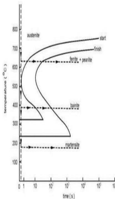
Gambar diagram Isothermal Transformation diagram
