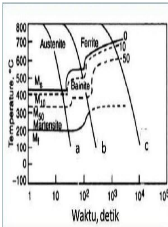
Gambar Continuous Cooling Transformation Diagram
