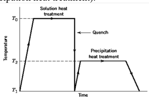
Gambar 1. Proses T6
